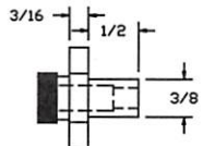
TRIM LEDGE TRIM GUIDE PART #TN1-38L PRICE-$39.00
