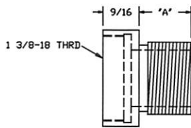
ROUTER GUIDE REDUCER RING PART #TNRR PRICE-$39.00
